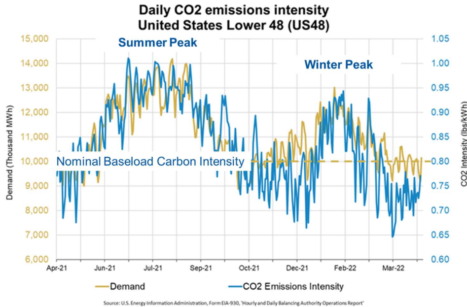
Figure 18: One-Year of US Electricity Demand and Generation CO 2 Intensity (DOE-EIA)
