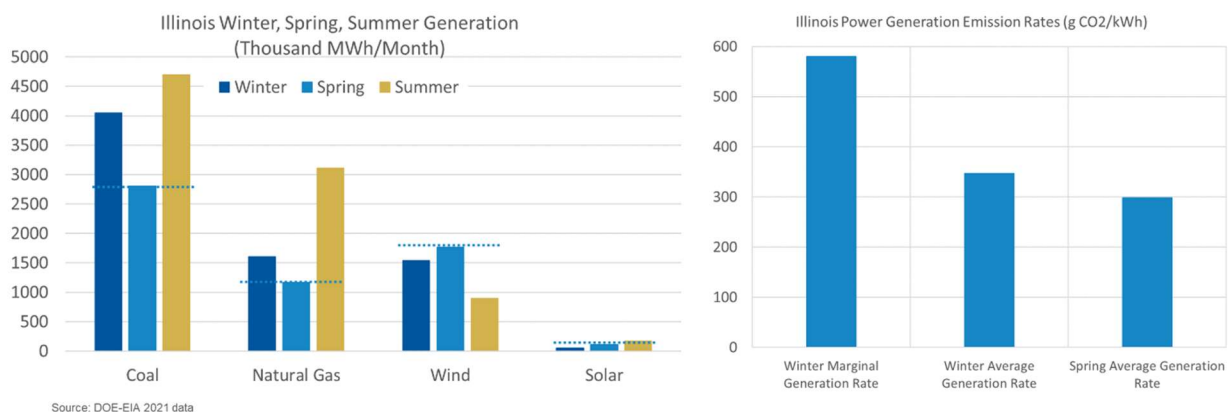
Figure 21: Illinois Winter Marginal, Winter and Spring Average CO 2 Generation Rates
