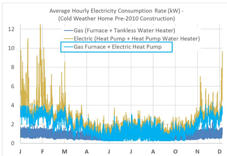
Figure 13: Hybrid Natural Gas and Electric Space Heating System Modeling (GTI; New York State home)
